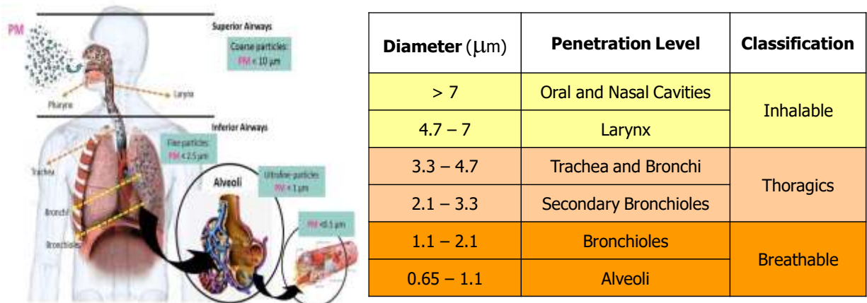
Figure 2 - Classification of particles according to the level of penetration into the respiratory system
