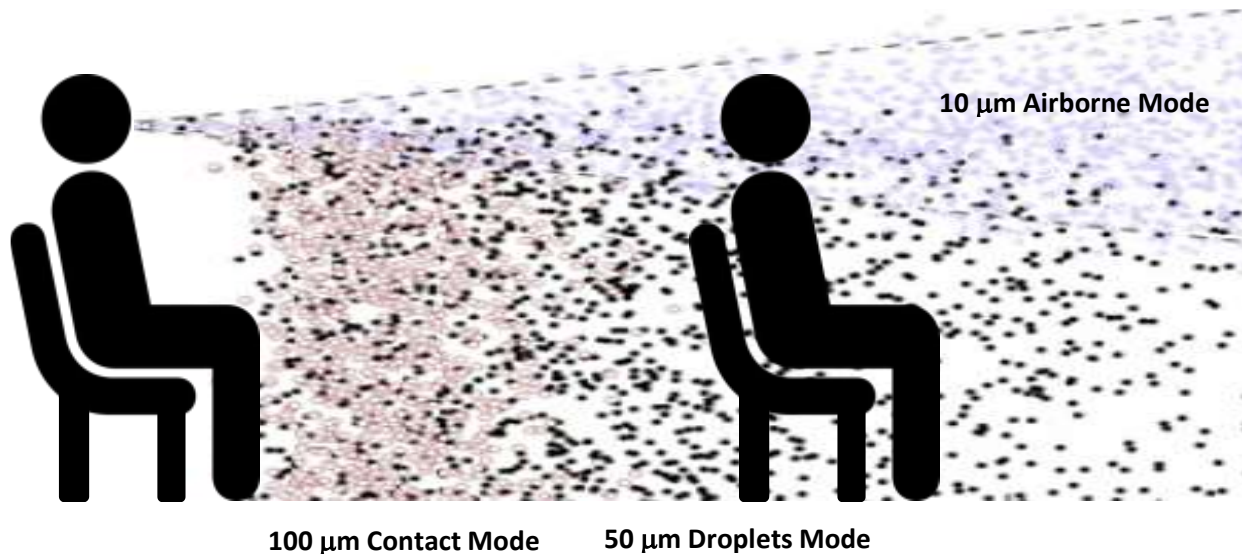
Figure 8 - Spatial zones potentially occupied by 10 \mu\text{m} , 50 \mu\text{m} and 100 \mu\text{m} particles exhaled by a person with a cough.(adapted from Jianjan Wei and Yuguo Li (2015))
