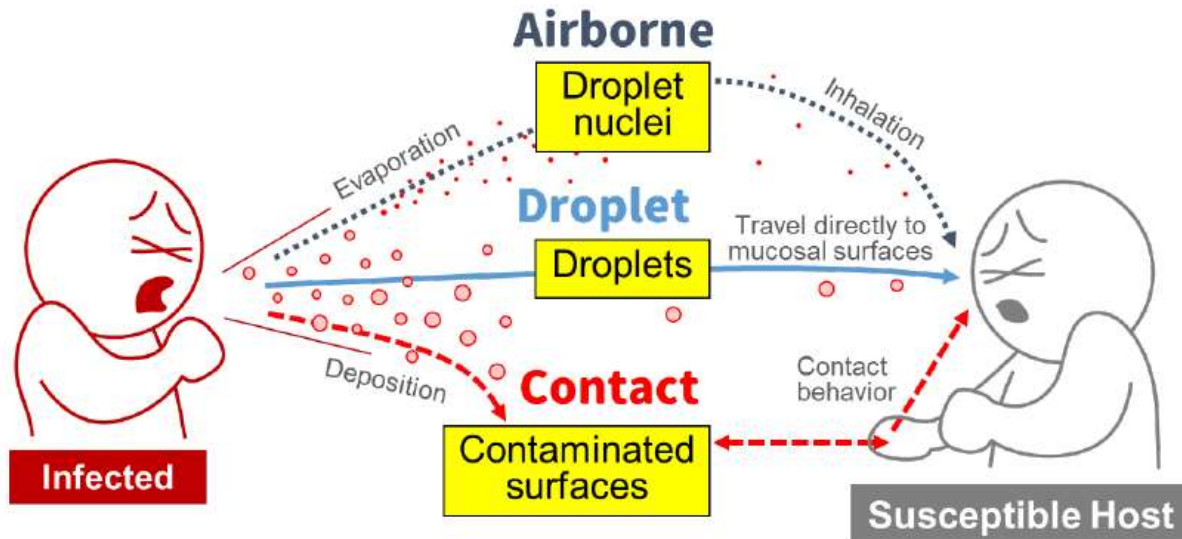
Figure 6 - Modes of Transmission from Exhaled Pathogens (adapted from leaflet of the Office of the Prime Minister and the Ministry of Health, Labor and Welfare of Japan (2020))
