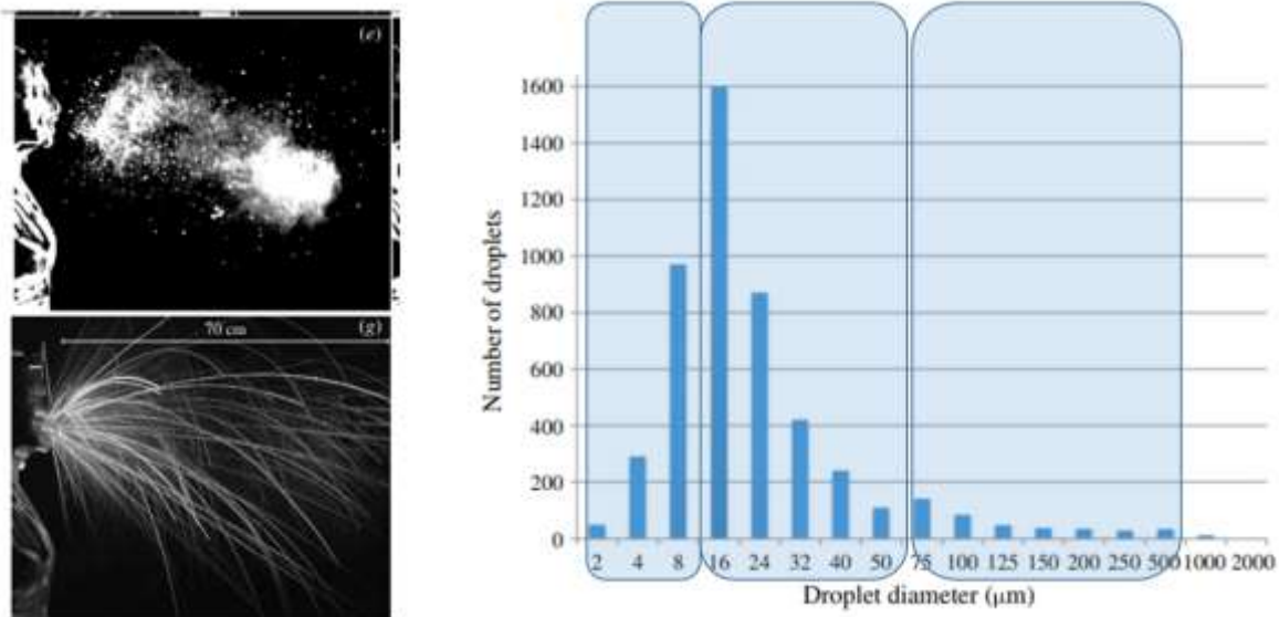
Figure 8 - Distribution by size classes of the drops exhaled in the cough
