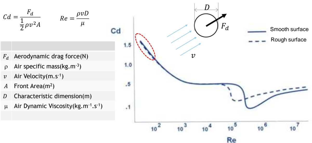
Figure 4 - Aerodynamic resistance coefficient as a function of Reynolds Number for a sphere
